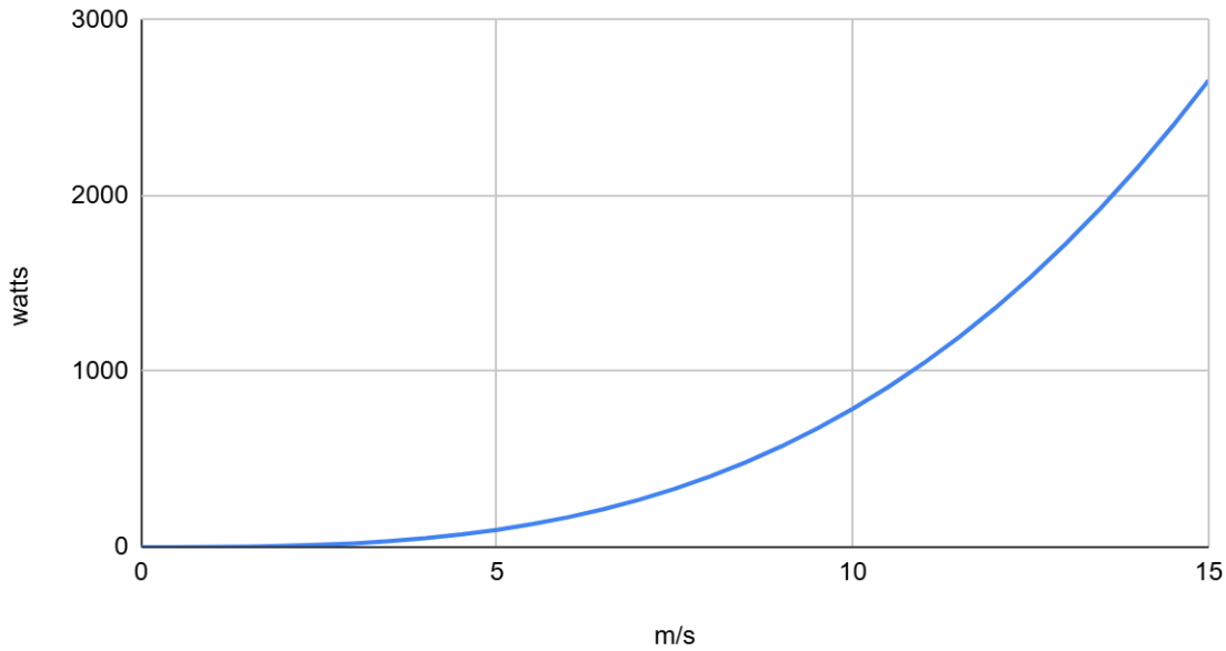
watts vs. m/s for 2m AL13 Power Tower
