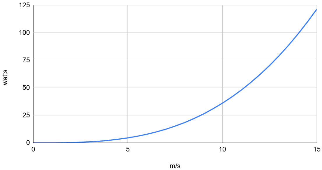
watts vs. m/s for 1m Tulip Turbine
