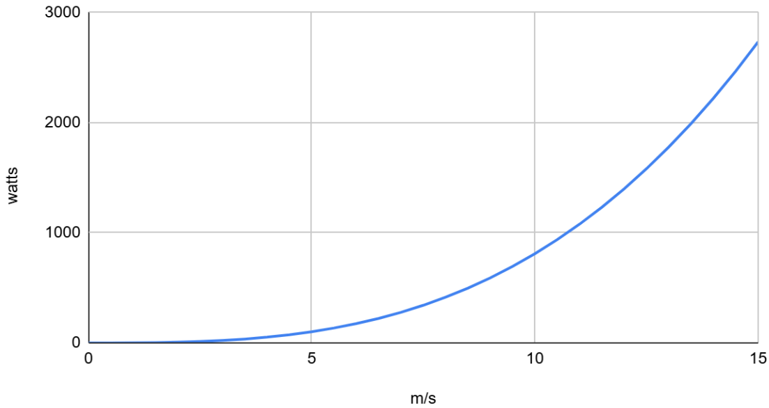
watts vs. m/s for 3m Tulip Turbine
