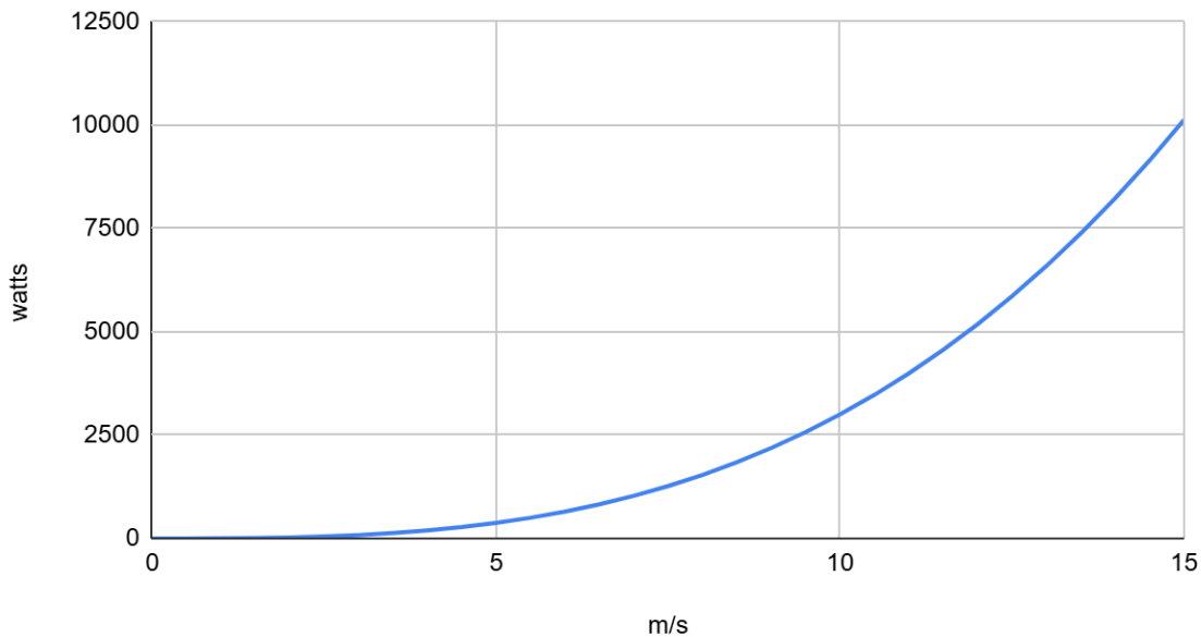
watts vs. m/s for 5m Tulip Turbine
