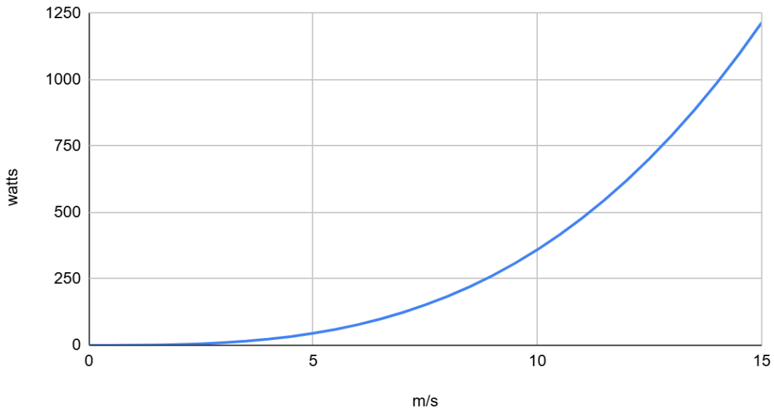
watts vs. m/s for 2m Tulip Turbine
