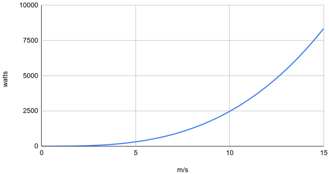
watts vs. m/s for 6m AL13 Power Tower
