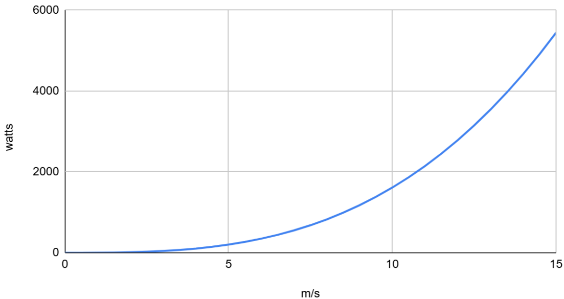
watts vs. m/s for 4m AL13 Power Tower
