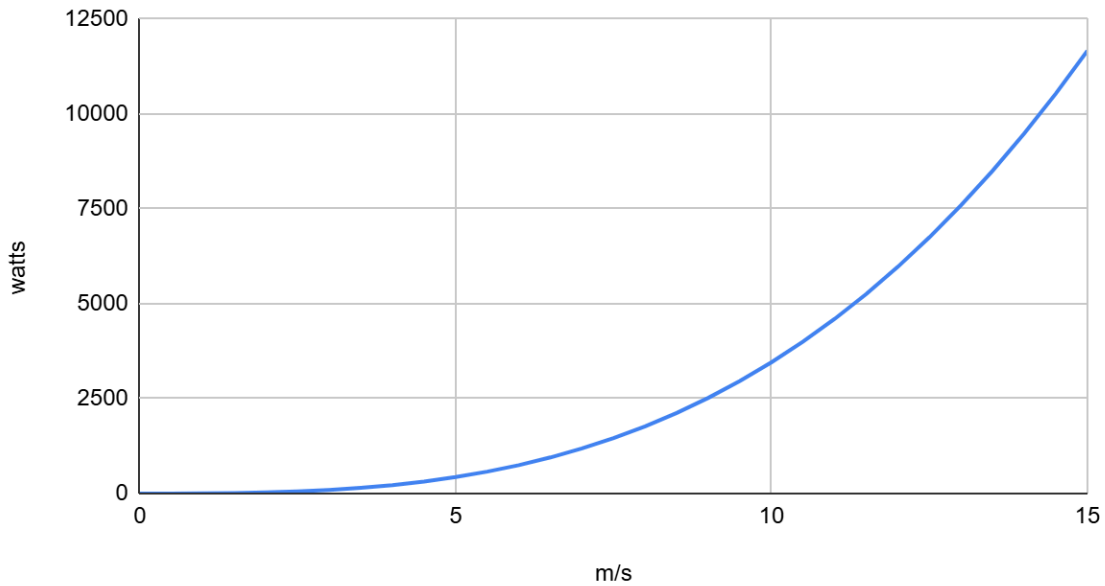
watts vs. m/s for 8m AL13 Power Tower
